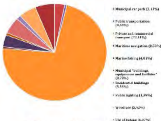
Figure 3 - Percentage distribution of GHG emissions by category
